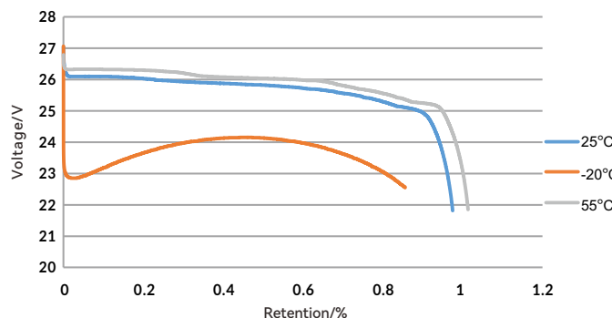
24V100Ah discharge curve at different temperatures
