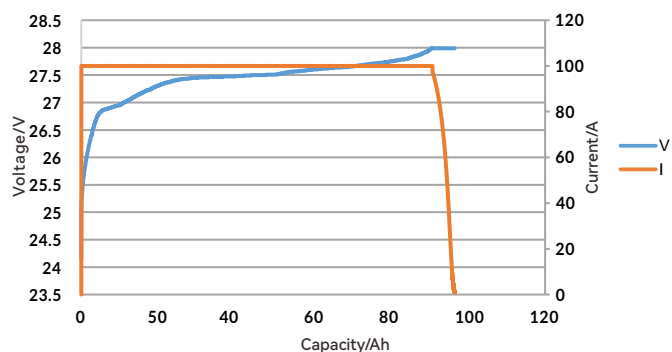
24V100Ah 1C Charge @RT
