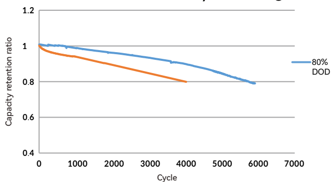
24V100Ah different DOD 0.2C cycle life curve @RT
