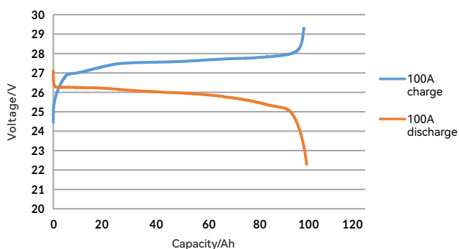
24V100Ah Charge-discharge capacity curve@RT
