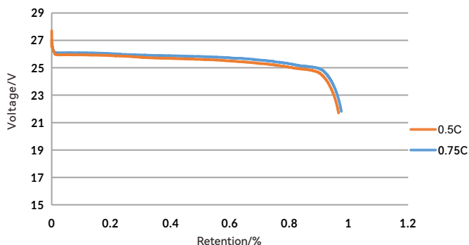
24V100Ah Discharge curve at different rates@RT
