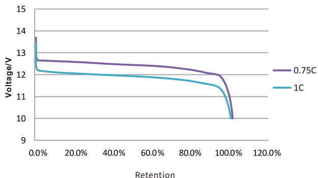
12V200Ah discharge curves at different rates@RT
